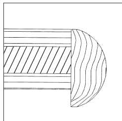
Bullnose-Drop External
