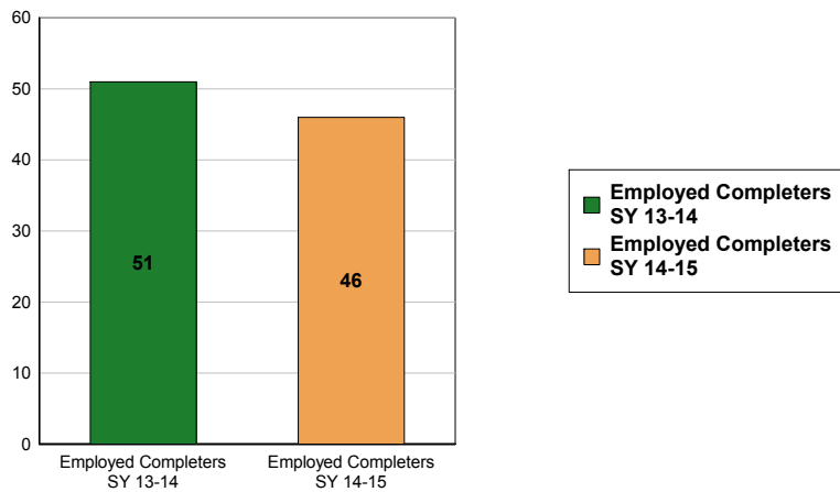
Persistence (2)
