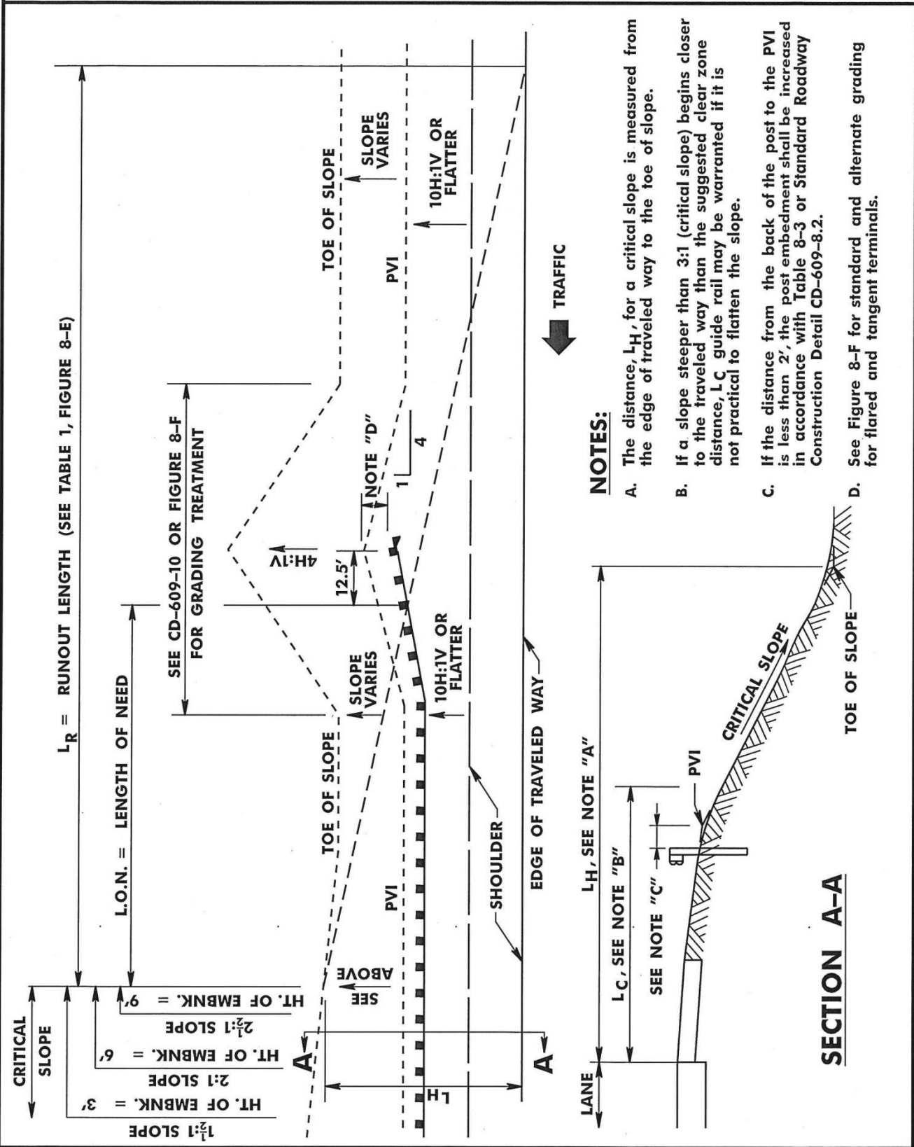
FIGURE 8-H: GUIDE RAIL TREATMENT FOR CRITICAL EMBANKMENT SLOPES
