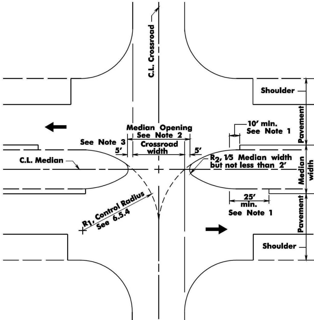
FIGURE 6-I: GRASS MEDIAN OPENING
