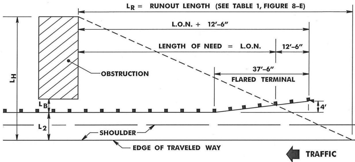
FIGURE 8-G: EXAMPLE OF APPROACH LENGTH OF NEED ON EMBANKMENT (FILL) SLOPES
