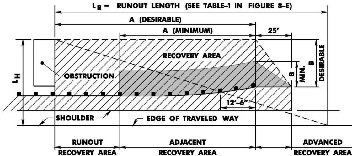
FIGURE 8-D: ROADSIDE RECOVERY AREA AT FLARED AND TANGENT TERMINALS
