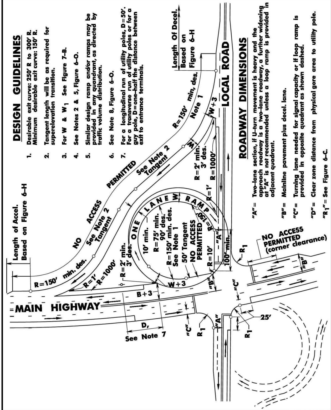
FIGURE 6-Q: TYPICAL TYPE "C" JUGHANDLE
