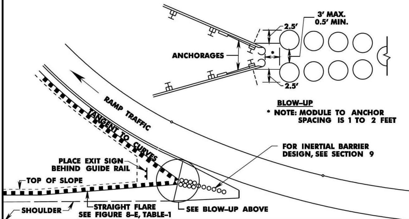
FIGURE 8-S: GUIDE RAIL TREATMENT EXAMPLES FOR LIMITED GORE AREAS
