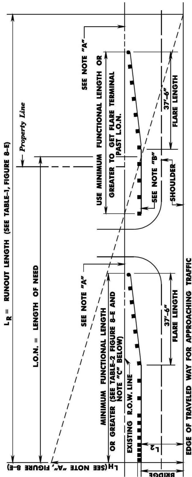
FIGURE 8-O: EXAMPLE OF GUIDE RAIL TREATMENT AT DRIVEWAY LOCATED WITHIN LENGTH OF NEED
