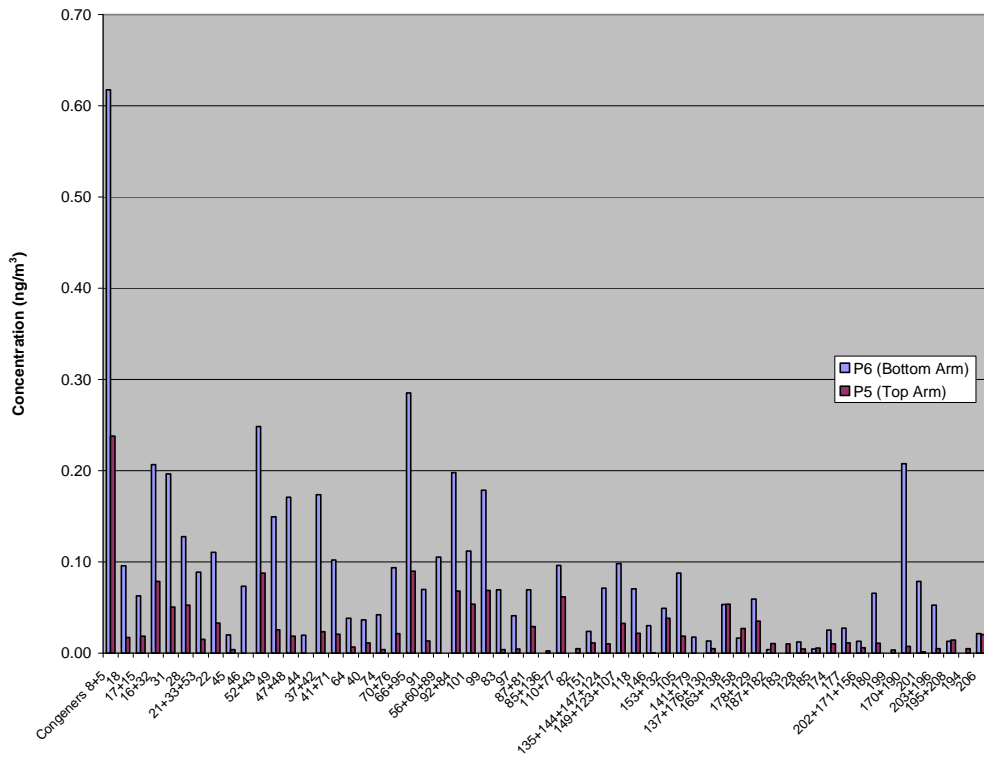
Figure 5. PCB congener mass distributions, October 23, 2001, afternoon.
