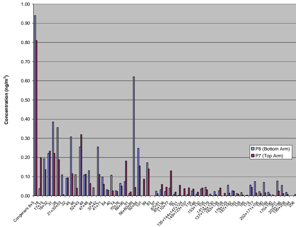
Figure 7. PCB congener mass distributions, October 24, 2001, nighttime.
