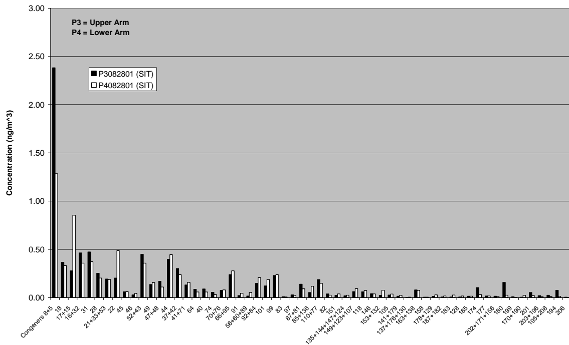
Figure 2. Nighttime PCB congener mass distributions, August 29, 2001.
